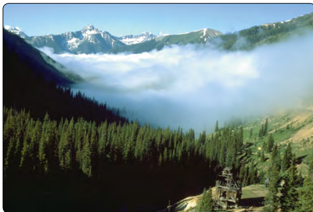
Figure 12-21. Radiation fog.
