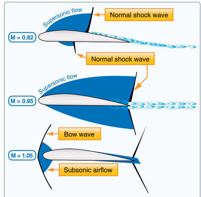
Figure 5-67. Shock waves.
