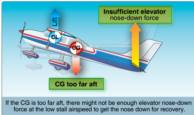
Vertical forces acting on an airplane in flight.
